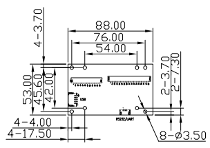
CONTROL BOARD T=MAX 7
